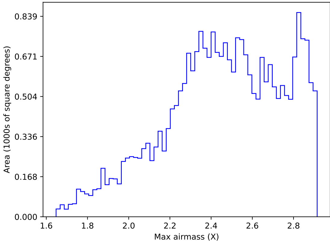
too_elab_r128_d3_ugrizy_v3.4_10yrs All sky i band: Max airmass
