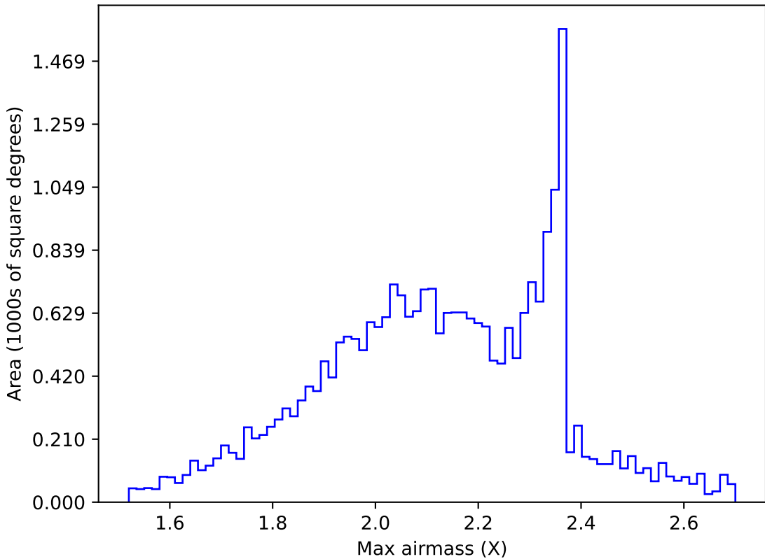
too_elab_r128_d3_ugrizy_v3.4_10yrs All sky g band: Max airmass
