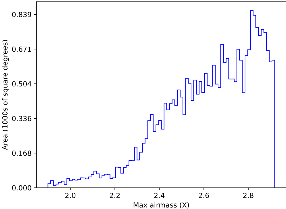
too_elab_r128_d3_ugrizy_v3.4_10yrs All sky all bands: Max airmass
