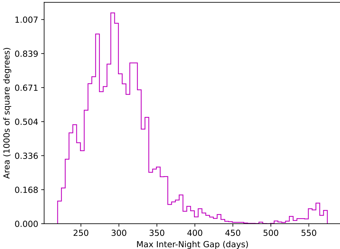
too_elab_r128_d3_ugrizzy_v3.4_10yrs WFD z band: Max Inter-Night Gap
