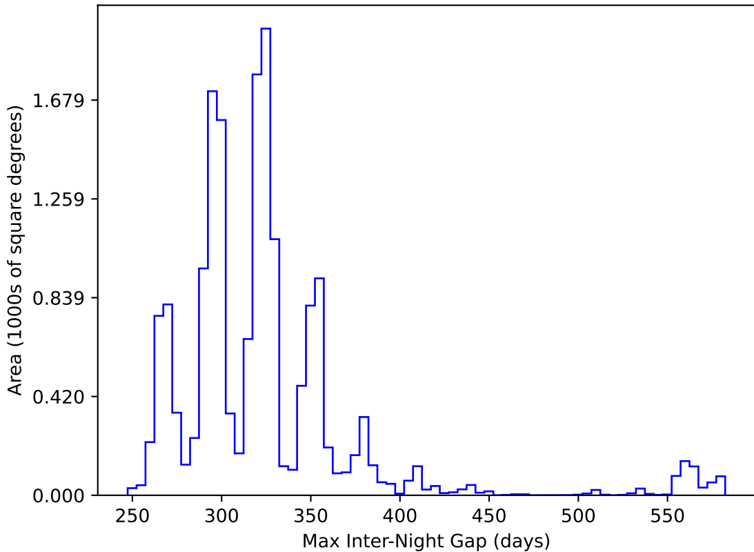
too_elab_r128_d3_ugrizy_v3.4_10yrs WFD y band: Max Inter-Night Gap
