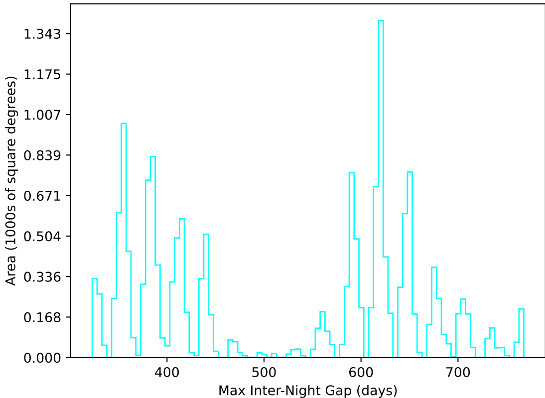
too_elab_r128_d3_ugrizy_v3.4_10yrs WFD u band: Max Inter-Night Gap
