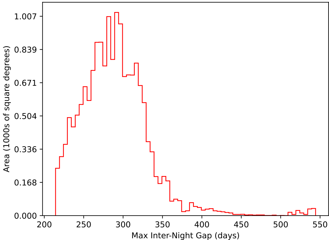
too_elab_r128_d3_ugrizy_v3.4_10yrs WFD i band: Max Inter-Night Gap
