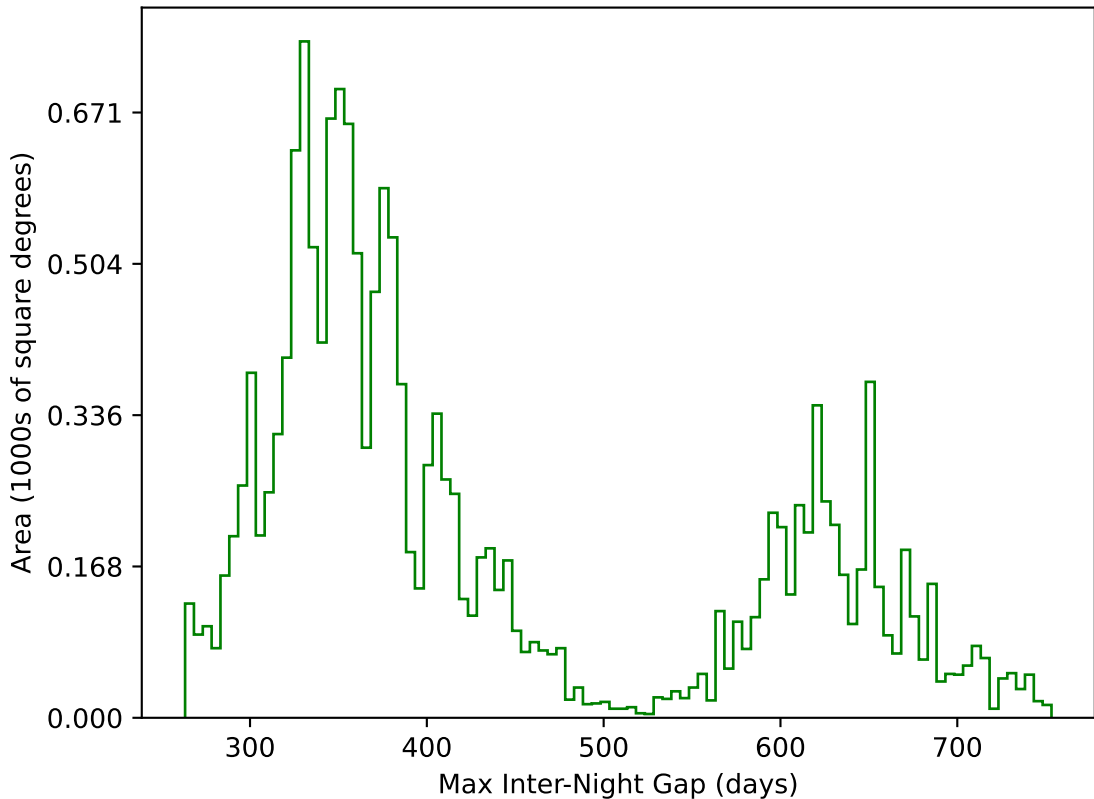
too_elab_r128_d3_ugrizy_v3.4_10yrs WFD g band: Max Inter-Night Gap
