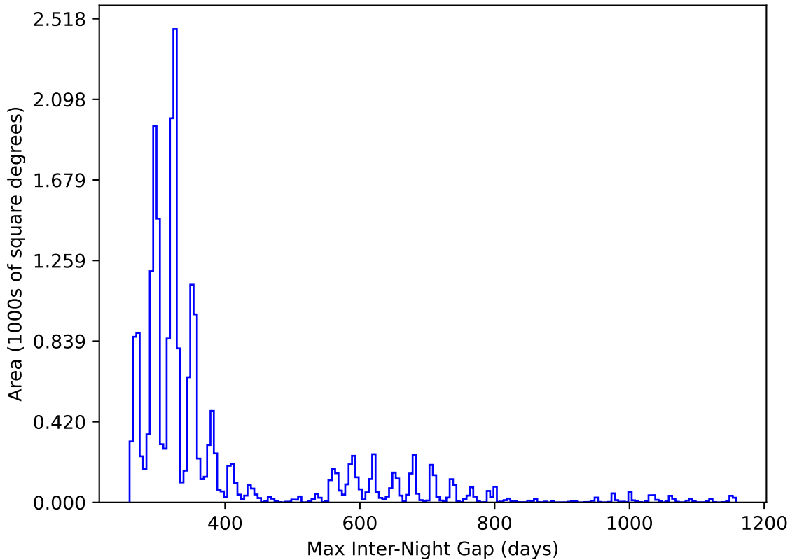
too_elab_r128_d3_ugrizy_v3.4_10yrs All sky y band: Max Inter-Night Gap
