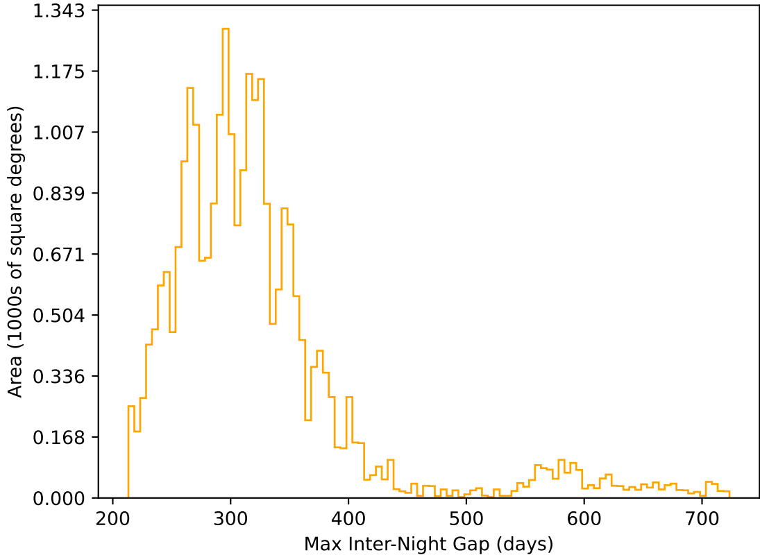
too_elab_r128_d3_ugrizy_v3.4_10yrs All sky r band: Max Inter-Night Gap
