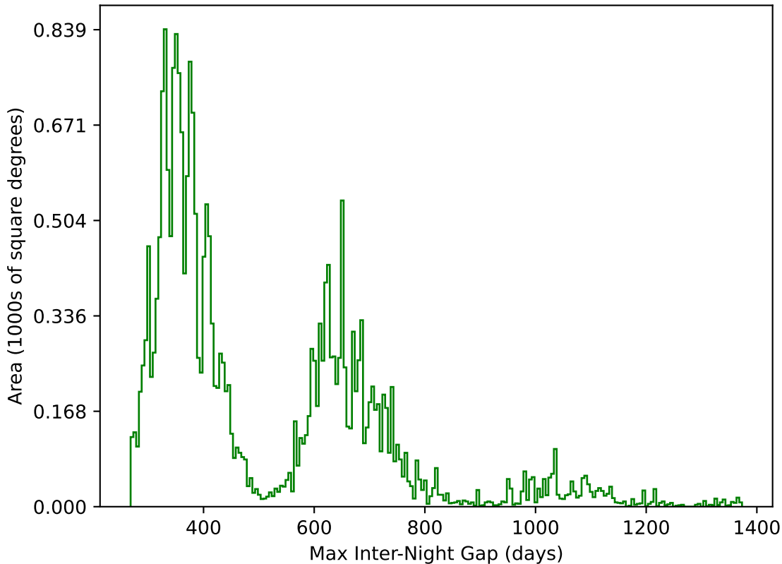
too_elab_r128_d3_ugrizy_v3.4_10yrs All sky g band: Max Inter-Night Gap
