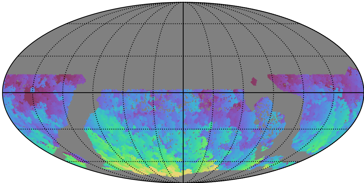
too_elab_r128_d3_ugrizy_v3.4_10yrs WFD u band: Max HA
