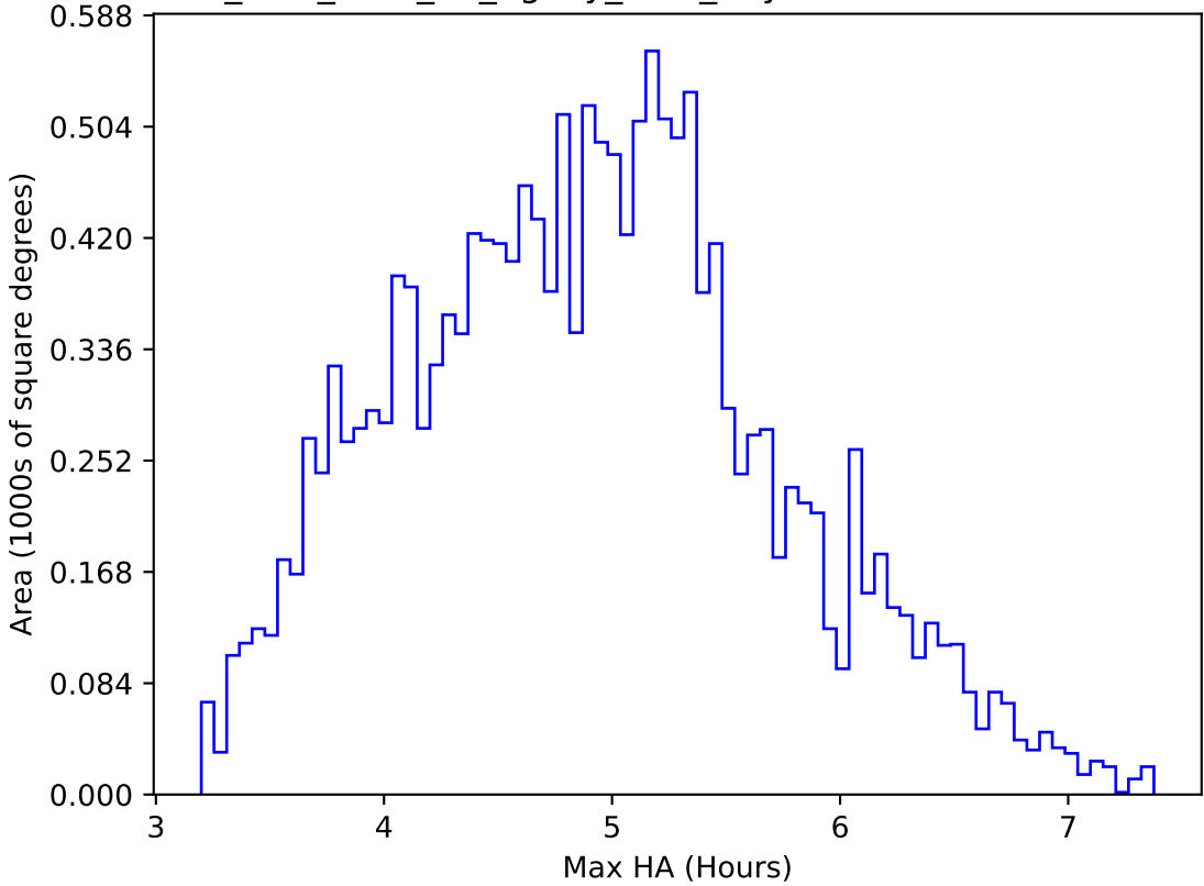
too_elab_r128_d3_ugrizy_v3.4_10yrs WFD i band: Max HA
