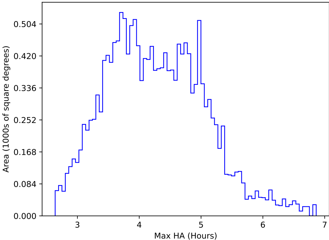
too_elab_r128_d3_ugrizy_v3.4_10yrs WFD g band: Max HA
