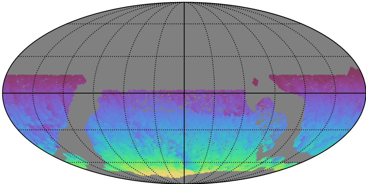
too_elab_r128_d3_ugrizy_v3.4_10yrs WFD all bands: Max HA
