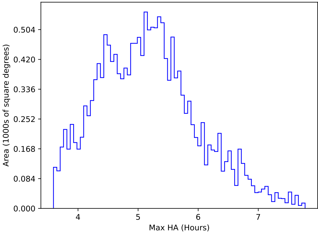
too_elab_r128_d3_ugrizy_v3.4_10yrs WFD all bands: Max HA
