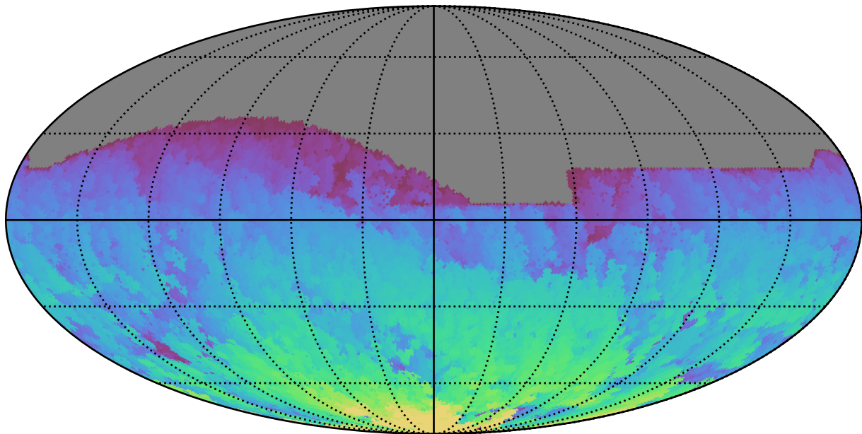
too_elab_r128_d3_ugrizy_v3.4_10yrs All sky z band: Max HA
