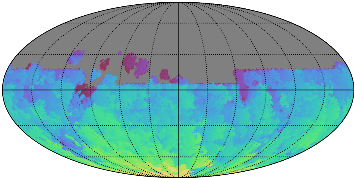
too_elab_r128_d3_ugrizy_v3.4_10yrs All sky u band: Max HA
