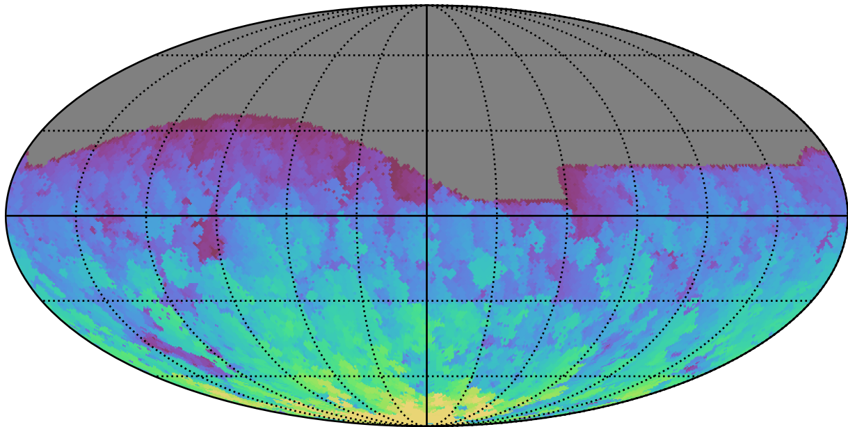
too_elab_r128_d3_ugrizy_v3.4_10yrs All sky g band: Max HA
