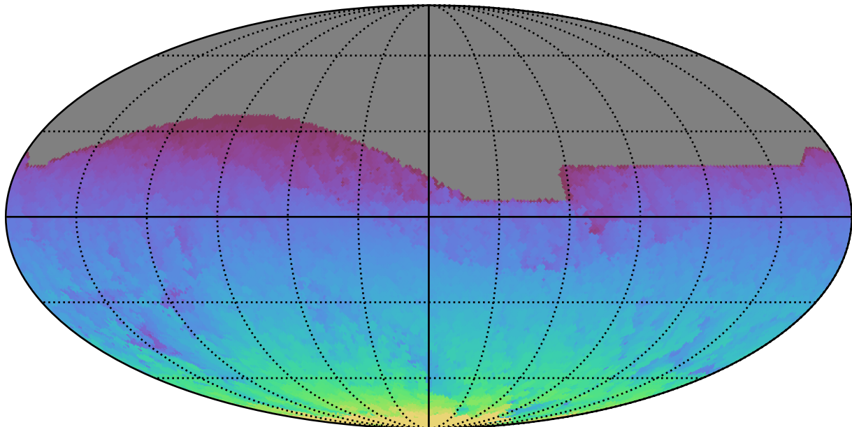
too_elab_r128_d3_ugrizy_v3.4_10yrs All sky all bands: Max HA
