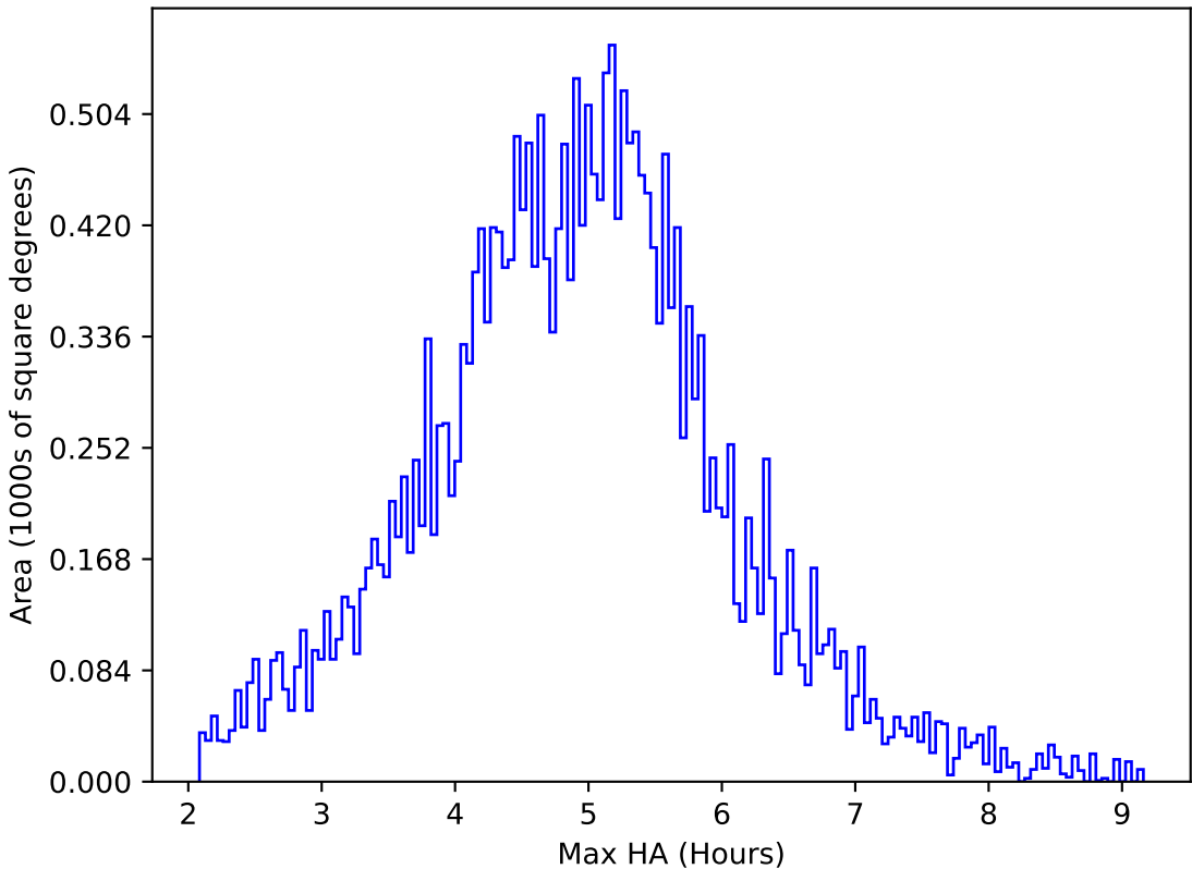
too_elab_r128_d3_ugrizy_v3.4_10yrs All sky all bands: Max HA
