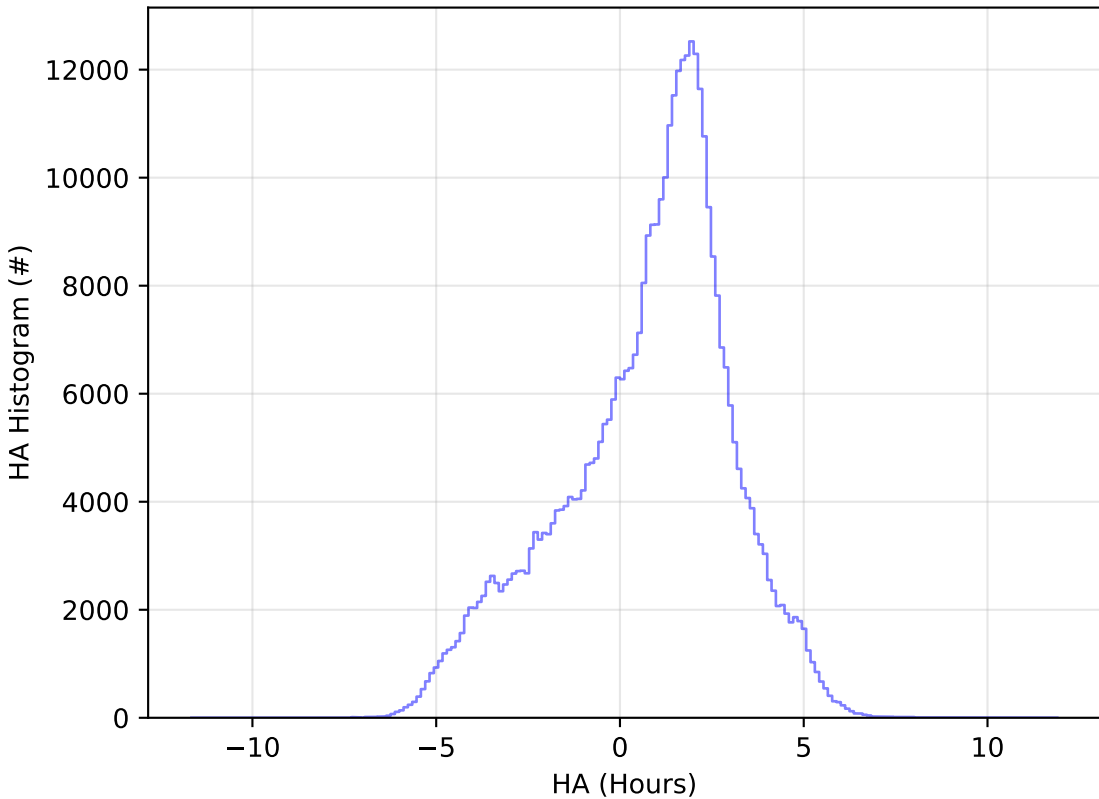
too_elab_r128_d3_ugrizy_v3.4_10yrs WFD z band: HA Histogram
