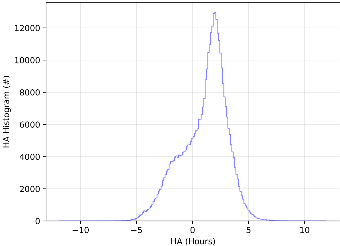
too_elab_r128_d3_ugrizy_v3.4_10yrs WFD y band: HA Histogram
