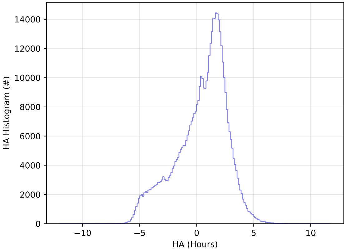
too_elab_r128_d3_ugrizy_v3.4_10yrs WFD r band: HA Histogram
