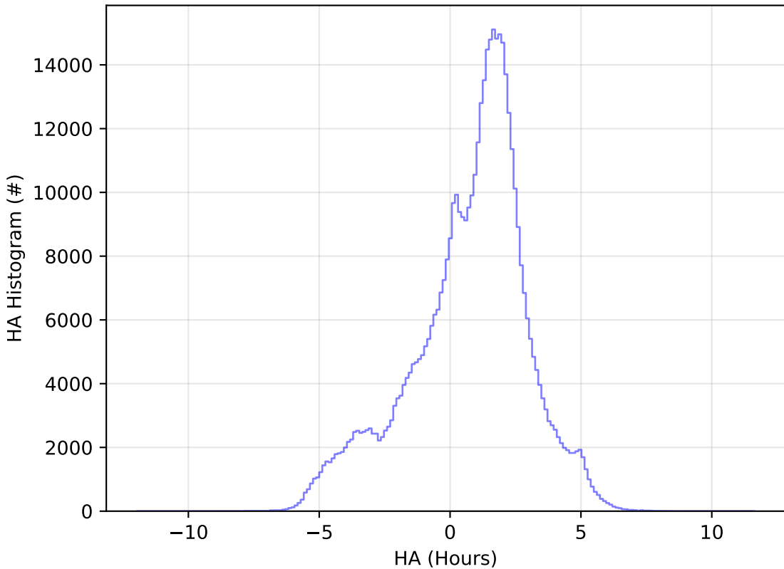
too_elab_r128_d3_ugrizy_v3.4_10yrs WFD i band: HA Histogram
