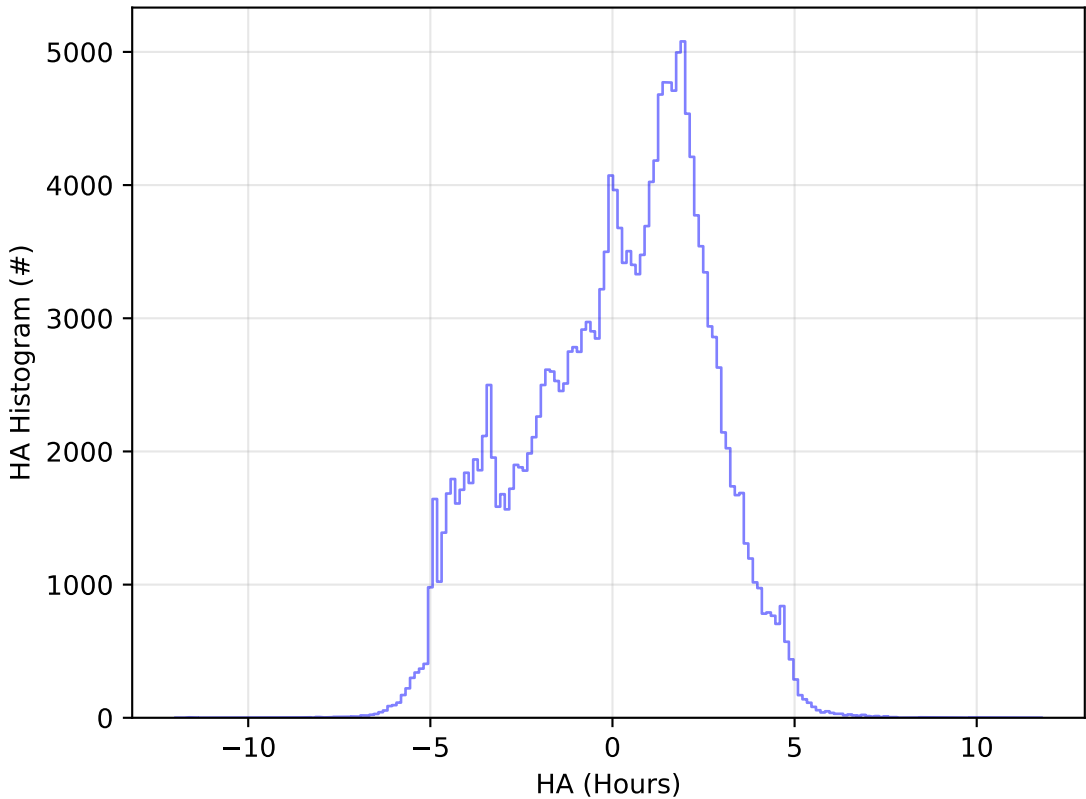
too_elab_r128_d3_ugrizy_v3.4_10yrs WFD g band: HA Histogram
