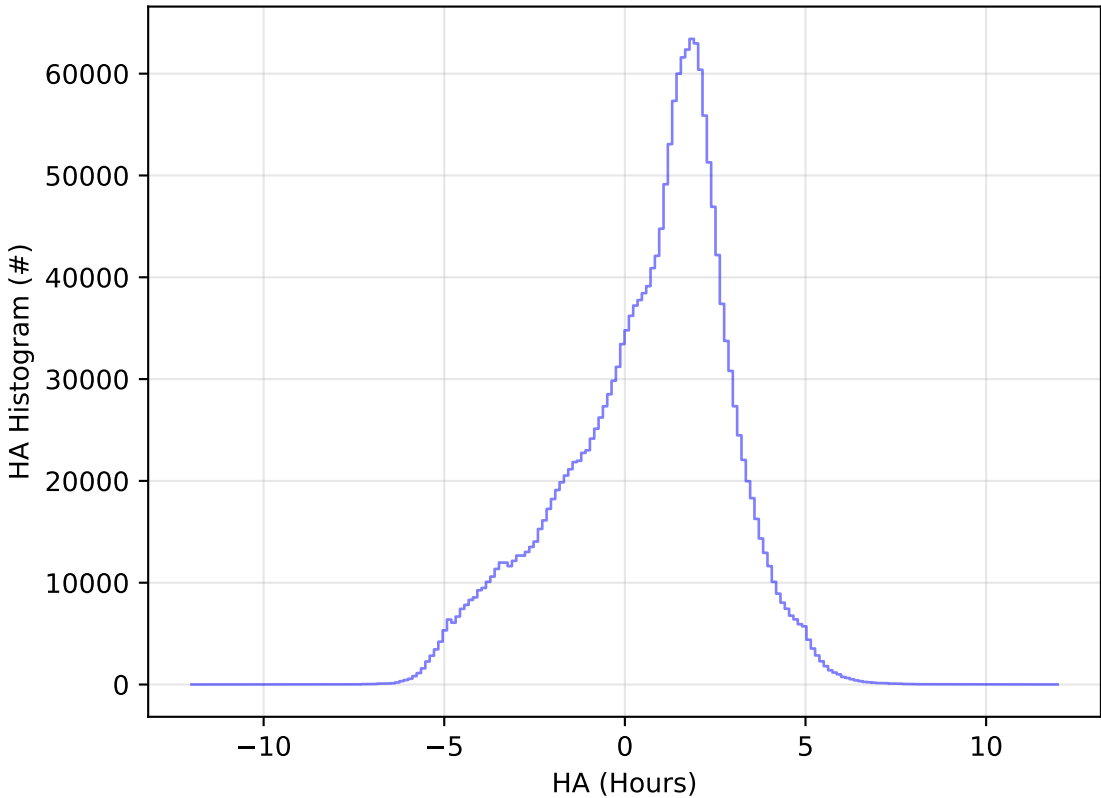
too_elab_r128_d3_ugrizy_v3.4_10yrs WFD all bands: HA Histogram
