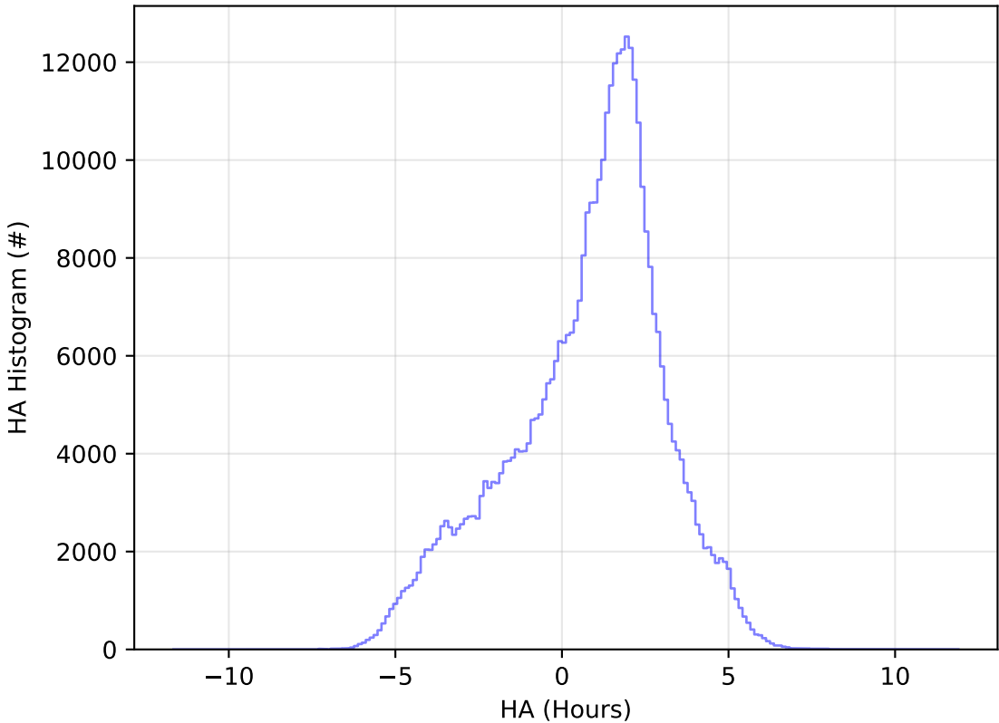
too_elab_r128_d3_ugrizy_v3.4_10yrs All sky z band: HA Histogram
