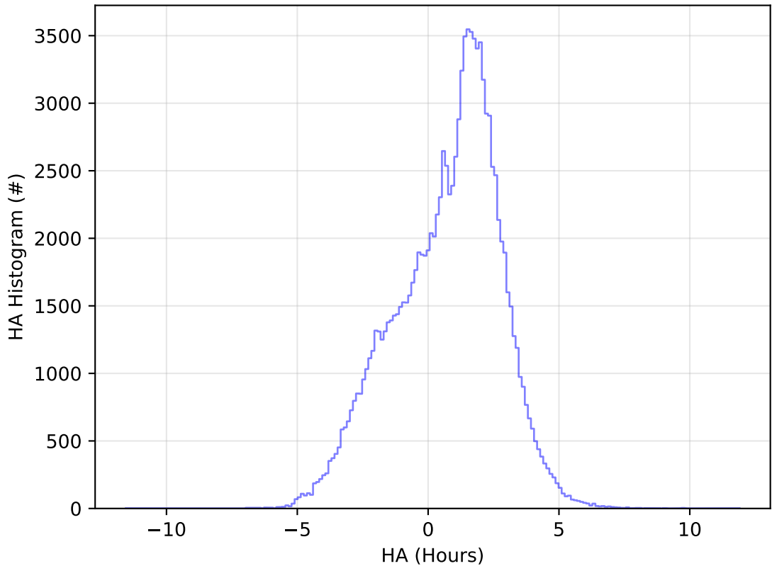
too_elab_r128_d3_ugrizy_v3.4_10yrs All sky u band: HA Histogram
