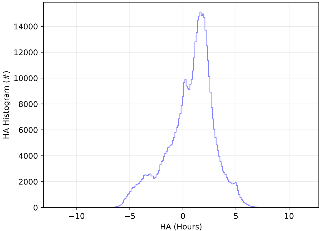
too_elab_r128_d3_ugrizy_v3.4_10yrs All sky i band: HA Histogram
