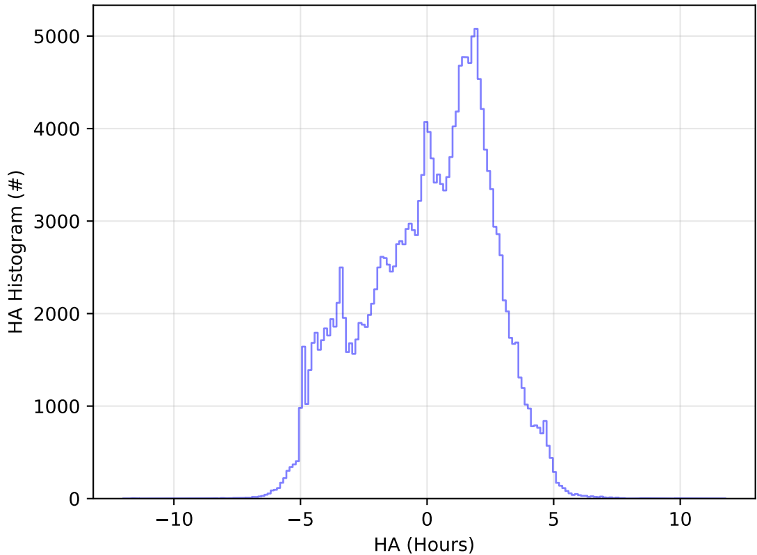
too_elab_r128_d3_ugrizy_v3.4_10yrs All sky g band: HA Histogram
