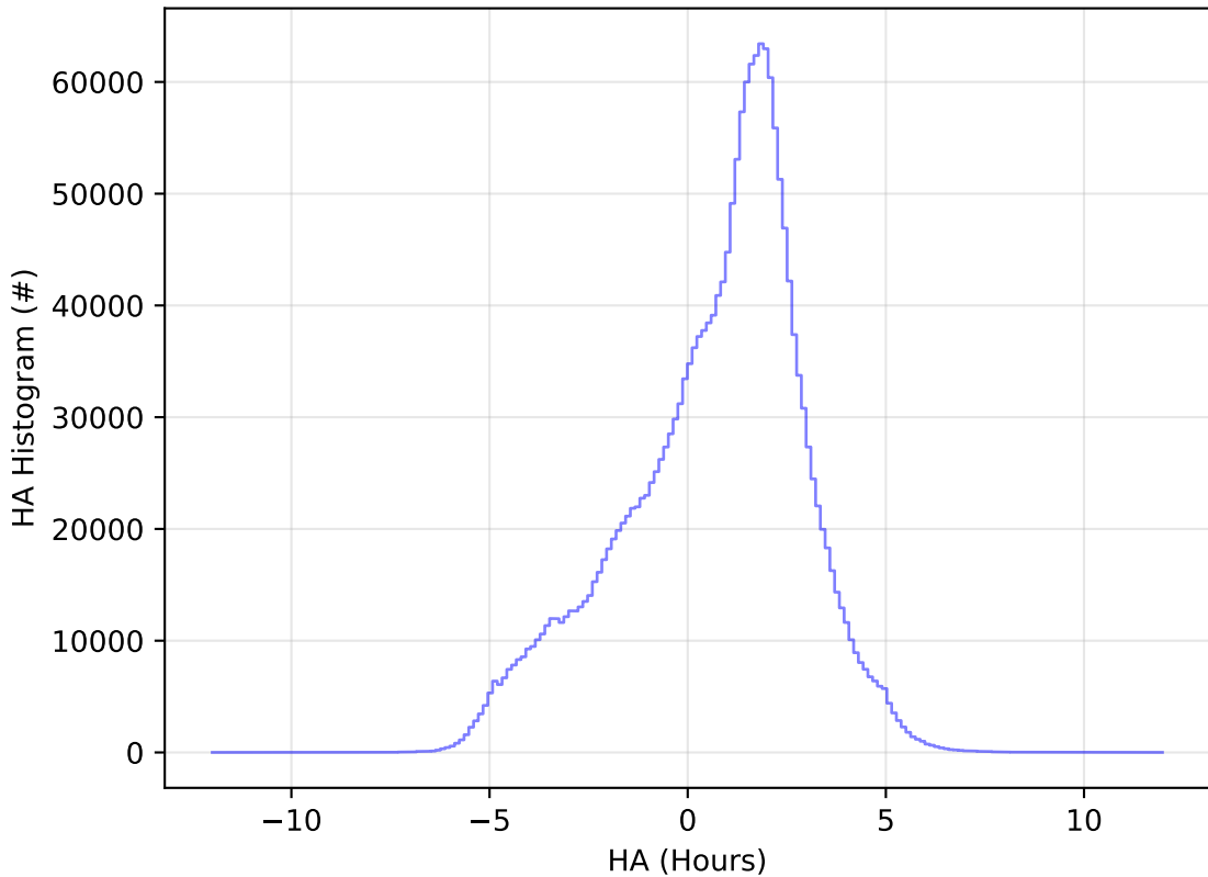
too_elab_r128_d3_ugrizy_v3.4_10yrs All sky all bands: HA Histogram
