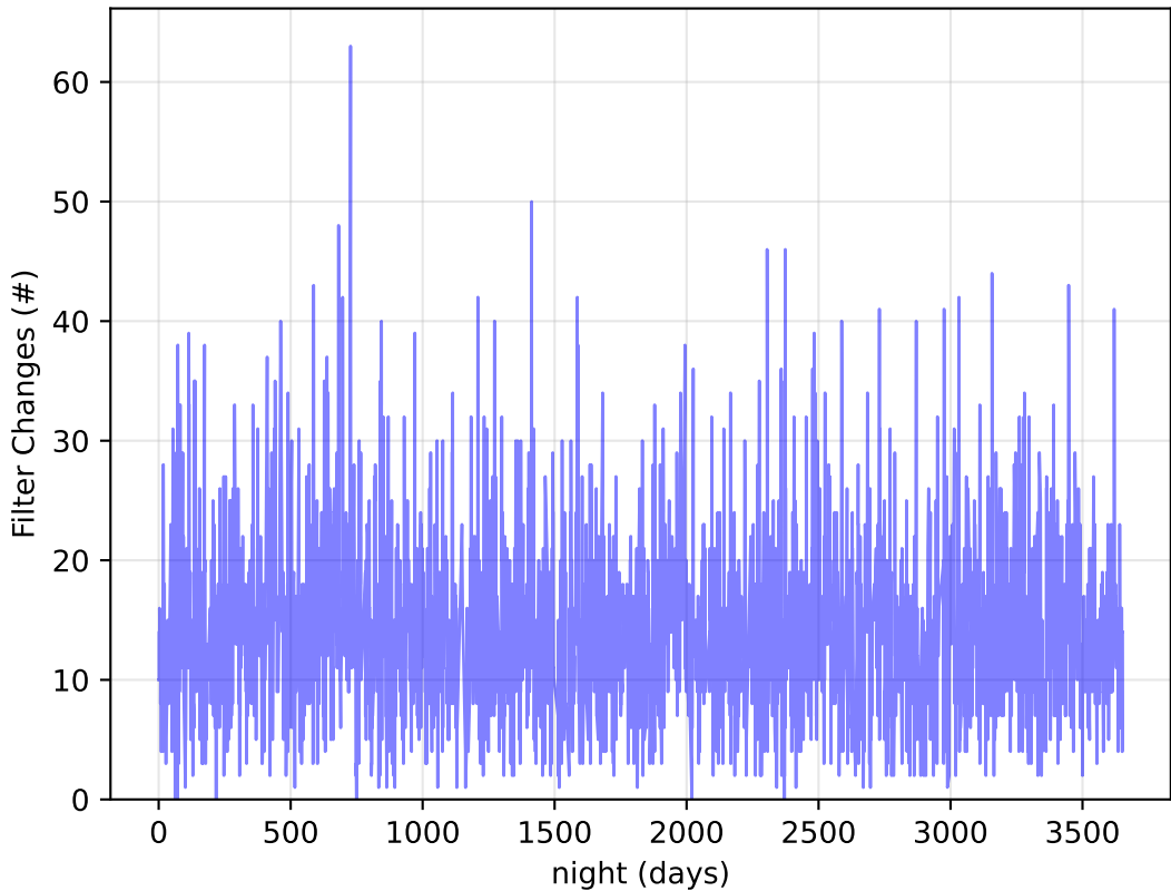
too_elab_r128_d3_ugrizy_v3.4_10yrs Per Night: Filter Changes
