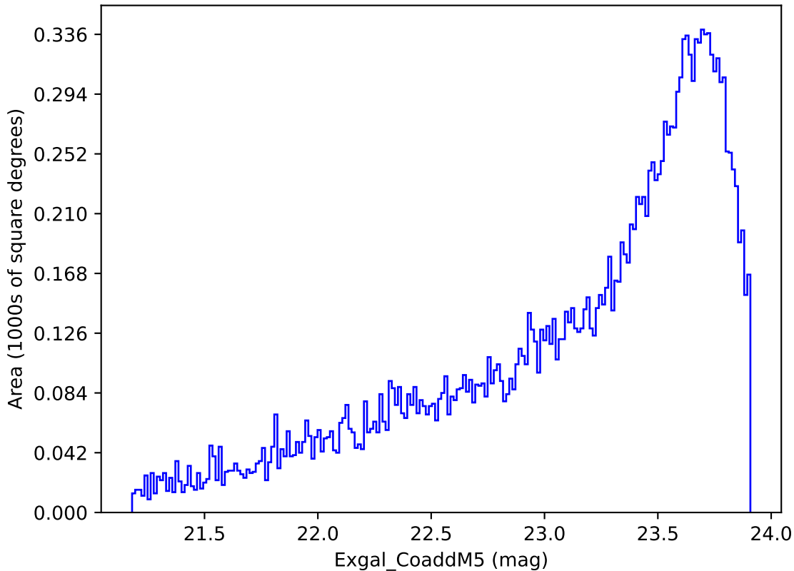
too_elab_r128_d3_ugrizy_v3.4_10yrs Yr 3-4 y band: Exgal_CoaddM5
