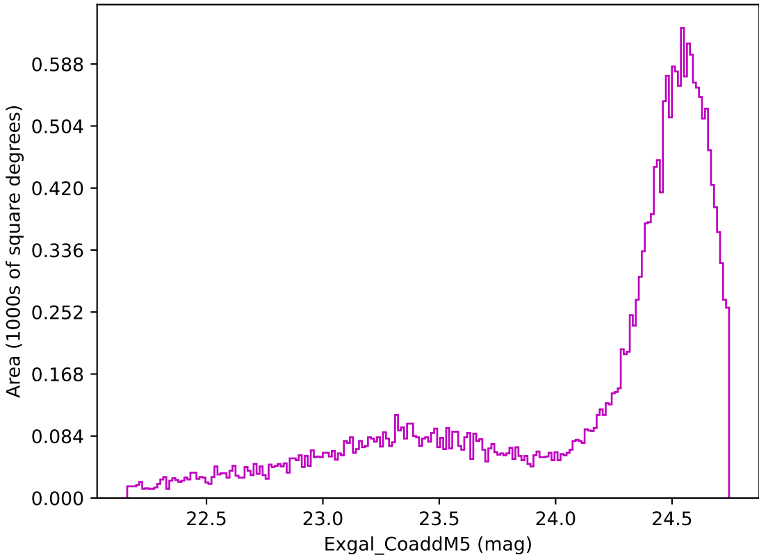
too_elab_r128_d3_ugrizy_v3.4_10yrs Yr 1 z band: Exgal_CoaddM5
