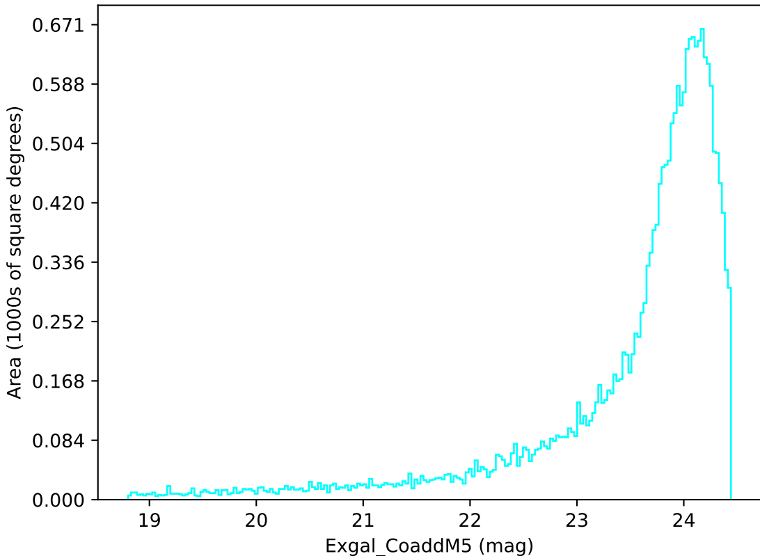
too_elab_r128_d3_ugrizy_v3.4_10yrs Yr 1 u band: Exgal_CoaddM5
