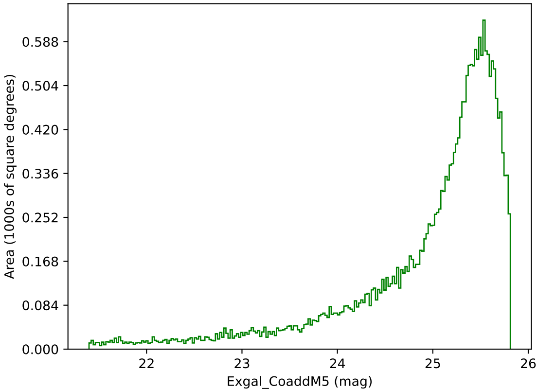
too_elab_r128_d3_ugrizy_v3.4_10yrs Yr 1 g band: Exgal_CoaddM5
