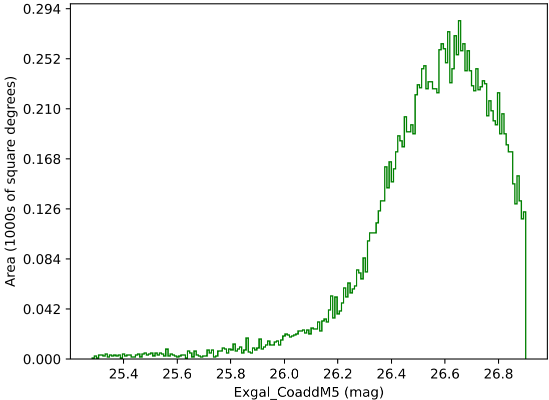
too_elab_r128_d3_ugrizy_v3.4_10yrs WFD g band: Exgal_CoaddM5
