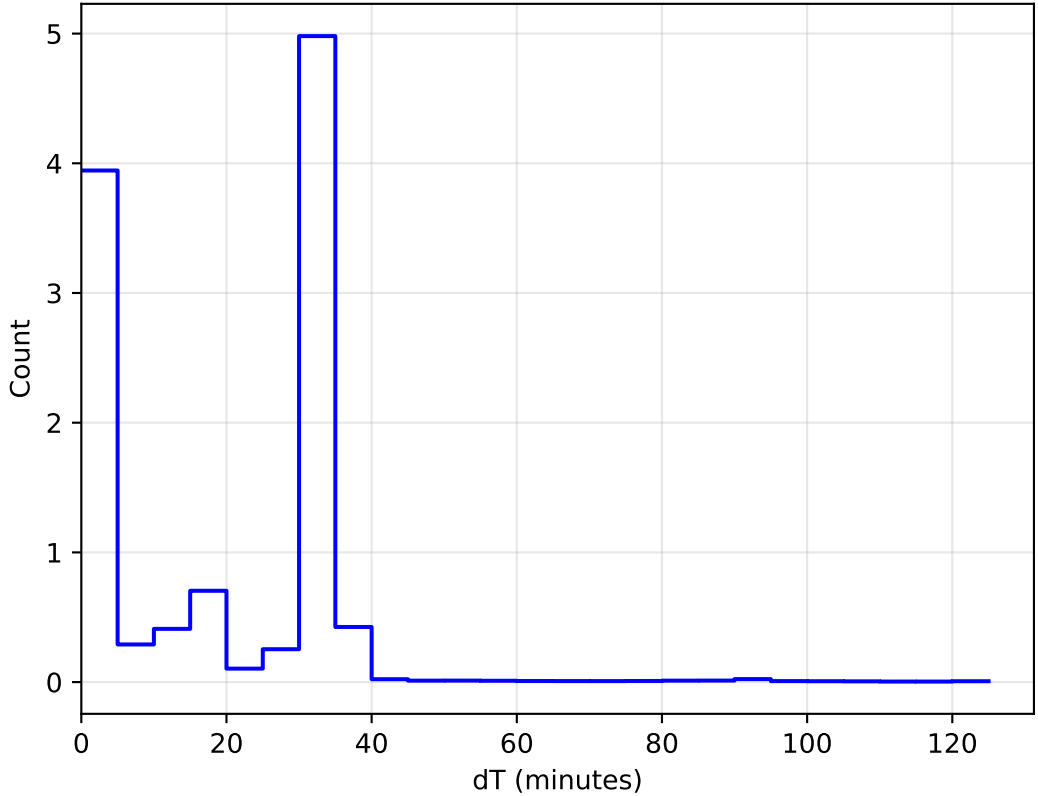
too_elab_r128_d3_ugrizy_v3.4_10yrs WFD: DeltaT Histogram 1e6
