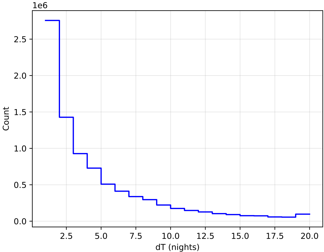
too_elab_r128_d3_ugrizy_v3.4_10yrs All sky all bands: DeltaNight Histogram
