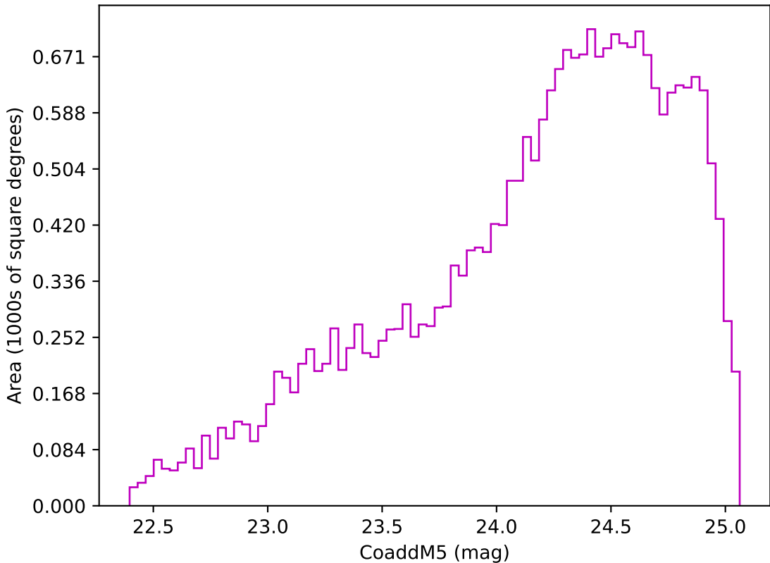
too_elab_r128_d3_ugrizy_v3.4_10yrs Yr 3-4 z band: CoaddM5
