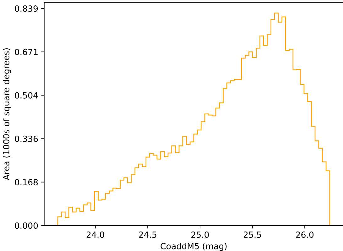
too_elab_r128_d3_ugrizy_v3.4_10yrs Yr 3-4 r band: CoaddM5
