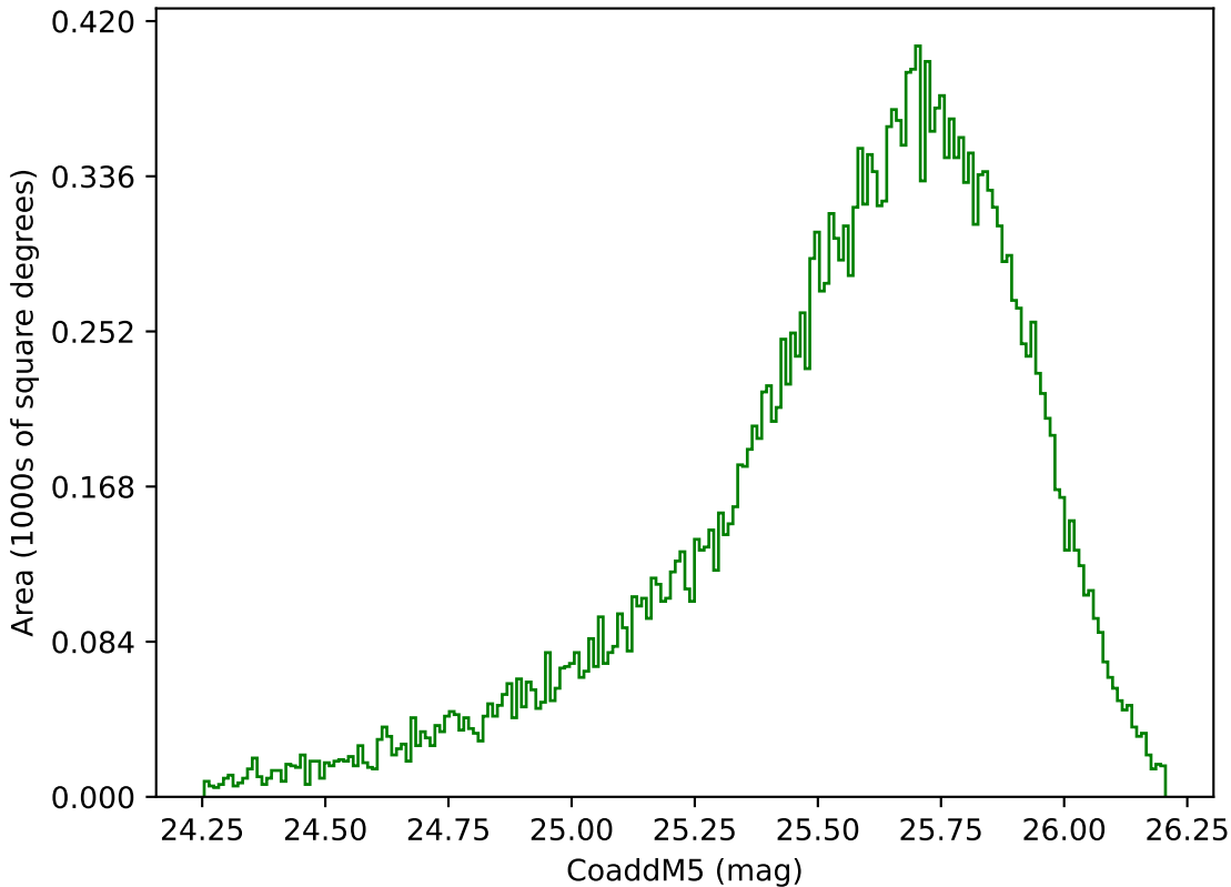
too_elab_r128_d3_ugrizy_v3.4_10yrs Yr 1 g band: CoaddM5
