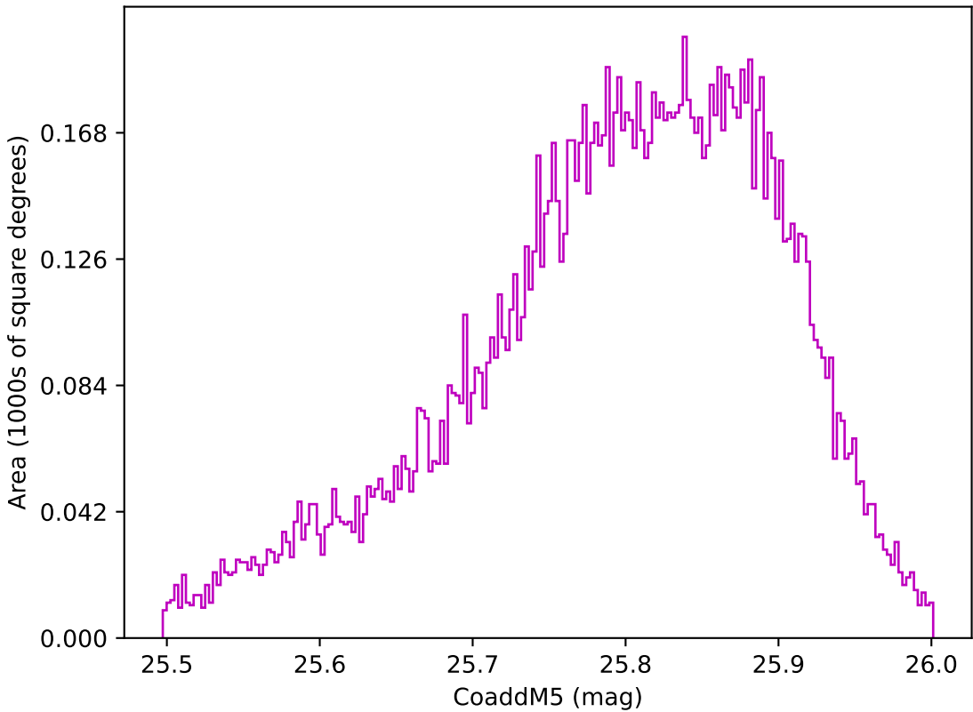
too_elab_r128_d3_ugrizy_v3.4_10yrs WFD z band: CoaddM5
