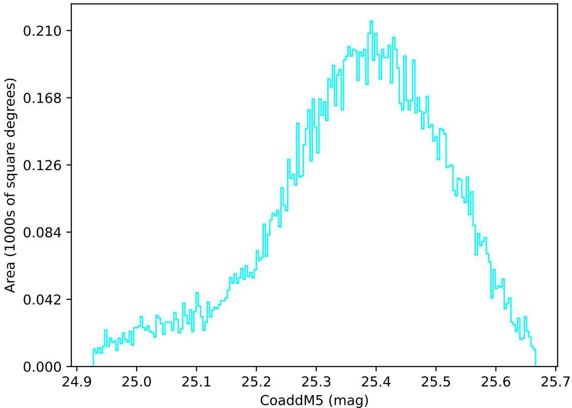
too_elab_r128_d3_ugrizy_v3.4_10yrs WFD u band: CoaddM5
