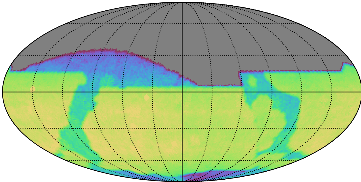
too_elab_r128_d3_ugrizy_v3.4_10yrs All sky z band: CoaddM5
