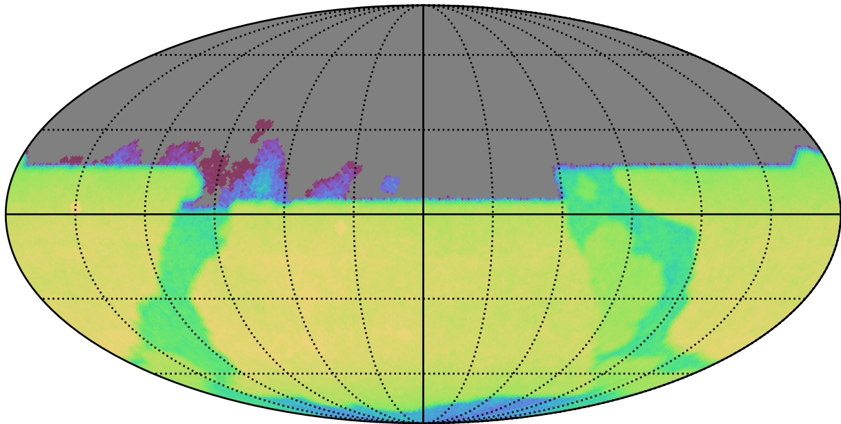
too_elab_r128_d3_ugrizy_v3.4_10yrs All sky y band: CoaddM5
