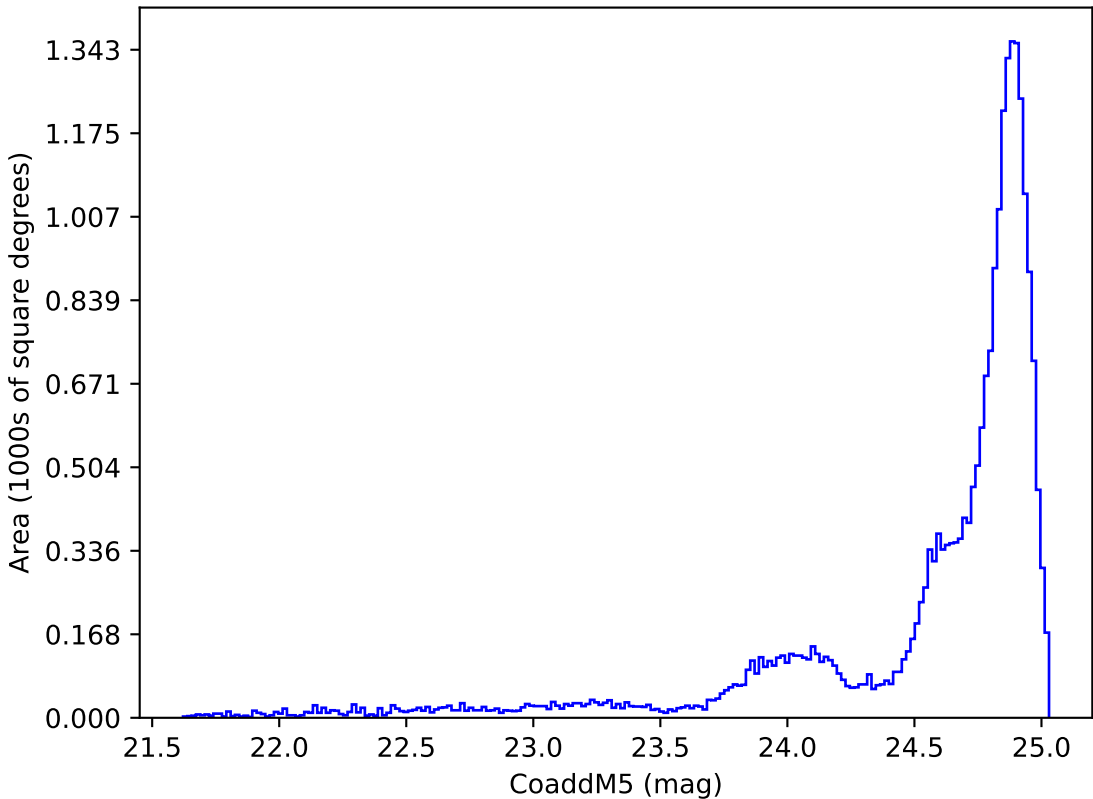
too_elab_r128_d3_ugrizy_v3.4_10yrs All sky y band: CoaddM5
