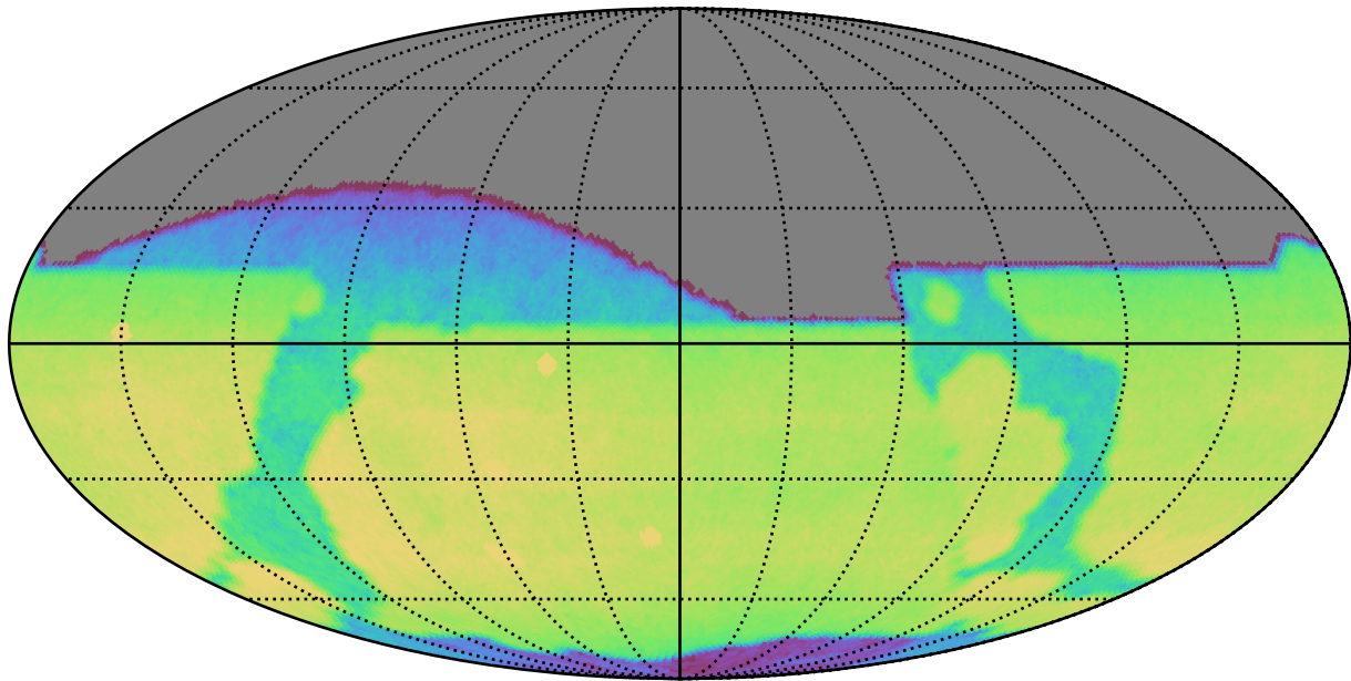
too_elab_r128_d3_ugrizy_v3.4_10yrs All sky r band: CoaddM5
