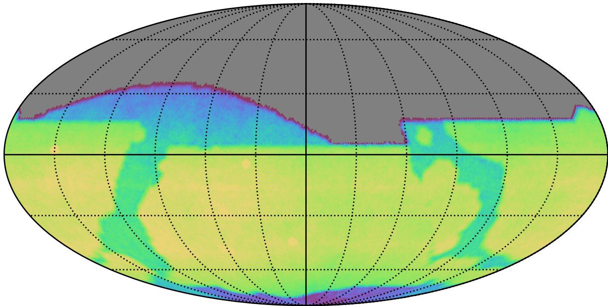
too_elab_r128_d3_ugrizy_v3.4_10yrs All sky i band: CoaddM5
